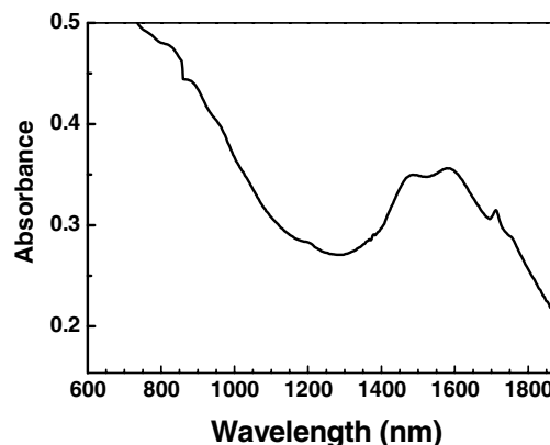
Fig. 4 Absorbance of the SWNTs-PVA film.
