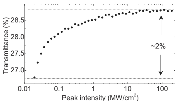
Transmittance as a function of peak intensity.
