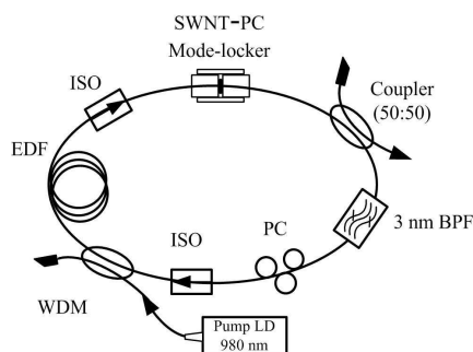
Fig. 2. Ring laser experimental setup.
