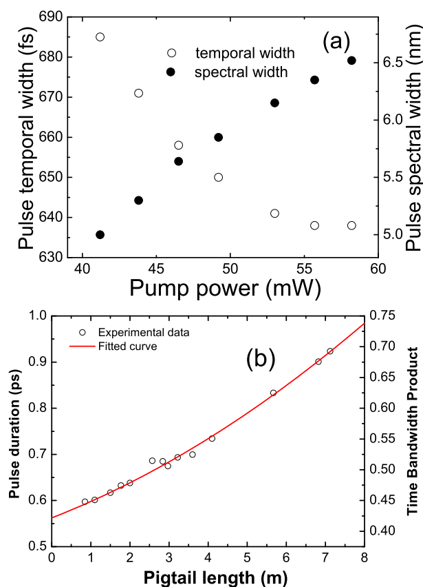
Figure 4 (a) Pulse spectral and temporal width as a function of pump power. (b) Pulse duration and time-bandwidth-product as a function of pigtail length.
